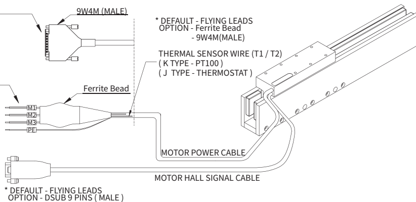
MOTOR CABLE WITH FLYING LEAD OR FERRITE BEAD OPTION
