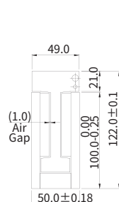
Standard Motor Coil
