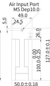
Air Cooled Motor Coil
