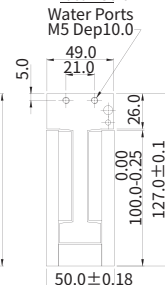
Water Cooled Motor Coil
